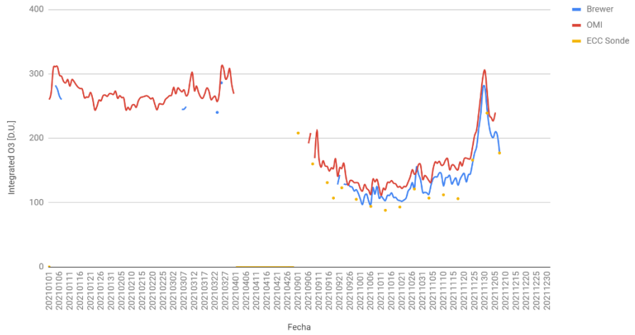
B099 vs OMI vs ECC Sonde
