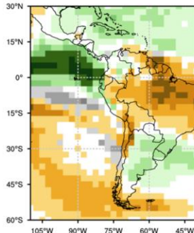
Probabilistic Multi-Model Ensemble Forecast Beijing,CMCC,CPTEC,Melbourne,Montreal,Moscow,Offenbach,Seoul
